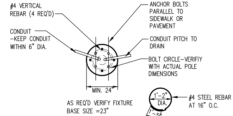
2 POLE BASE DETAIL E1.1 NOT TO SCALE
