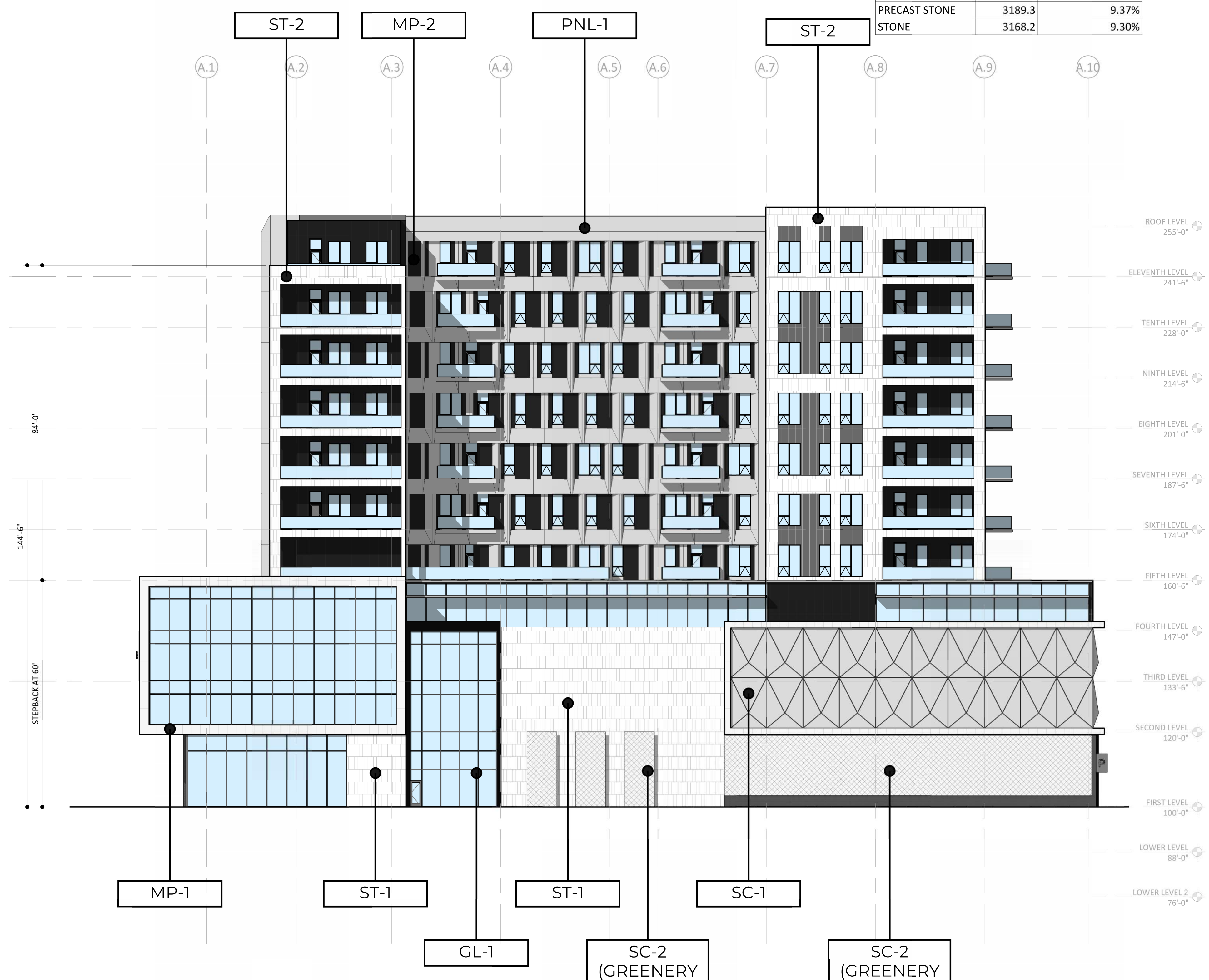
1 A106 SOUTH BUILDING ELEVATION 1/16" = 1'-0"
