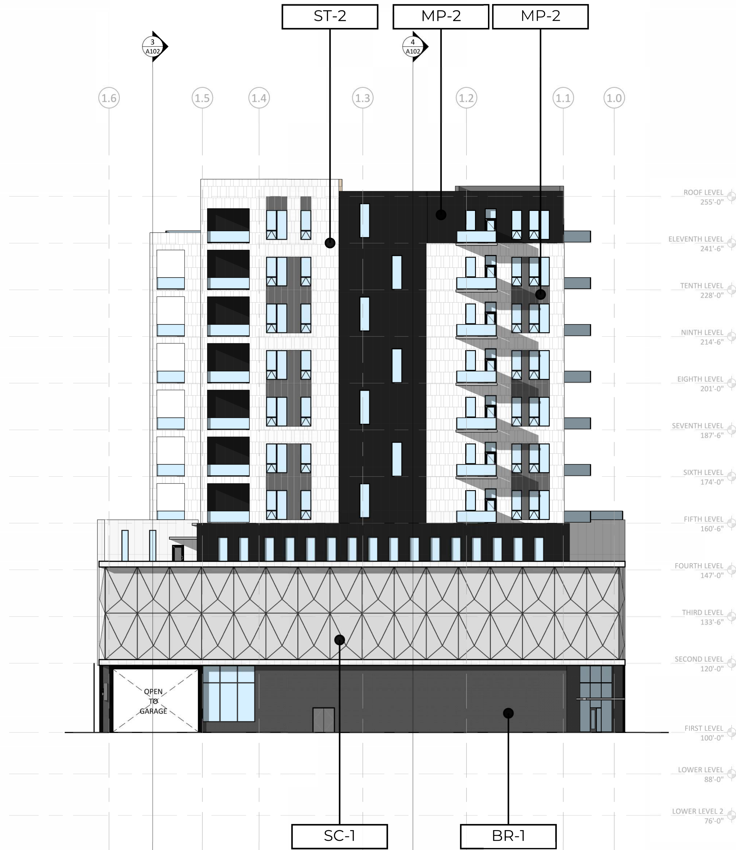
2 A107 EAST BUILDING ELEVATION 1/16" = 1'-0"
